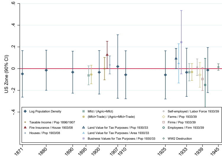
\theta in equation (2)
