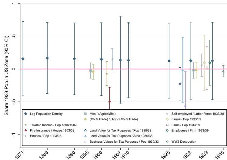
\delta in equation (2)
